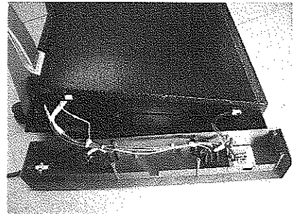
Internal view for GYD-15S
